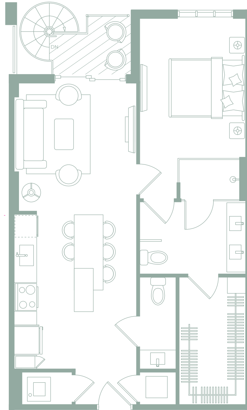
LEVEL 2
