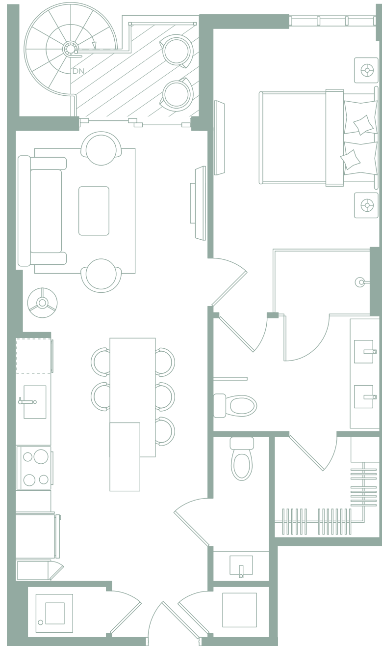
LEVEL 2
