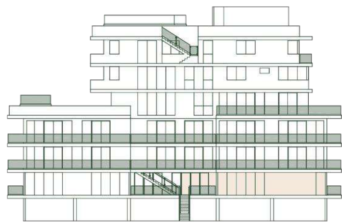
EAST FACADE
