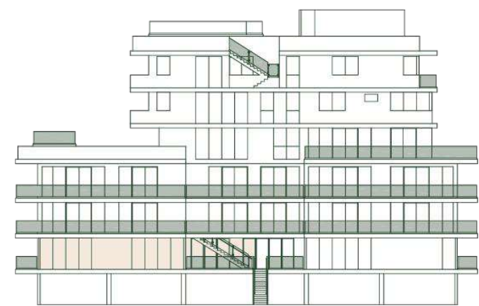
EAST FACADE
